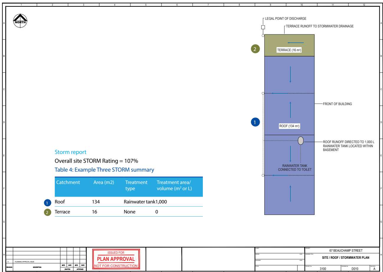
Figure 4: Example Three – Commercial site layout plan.
