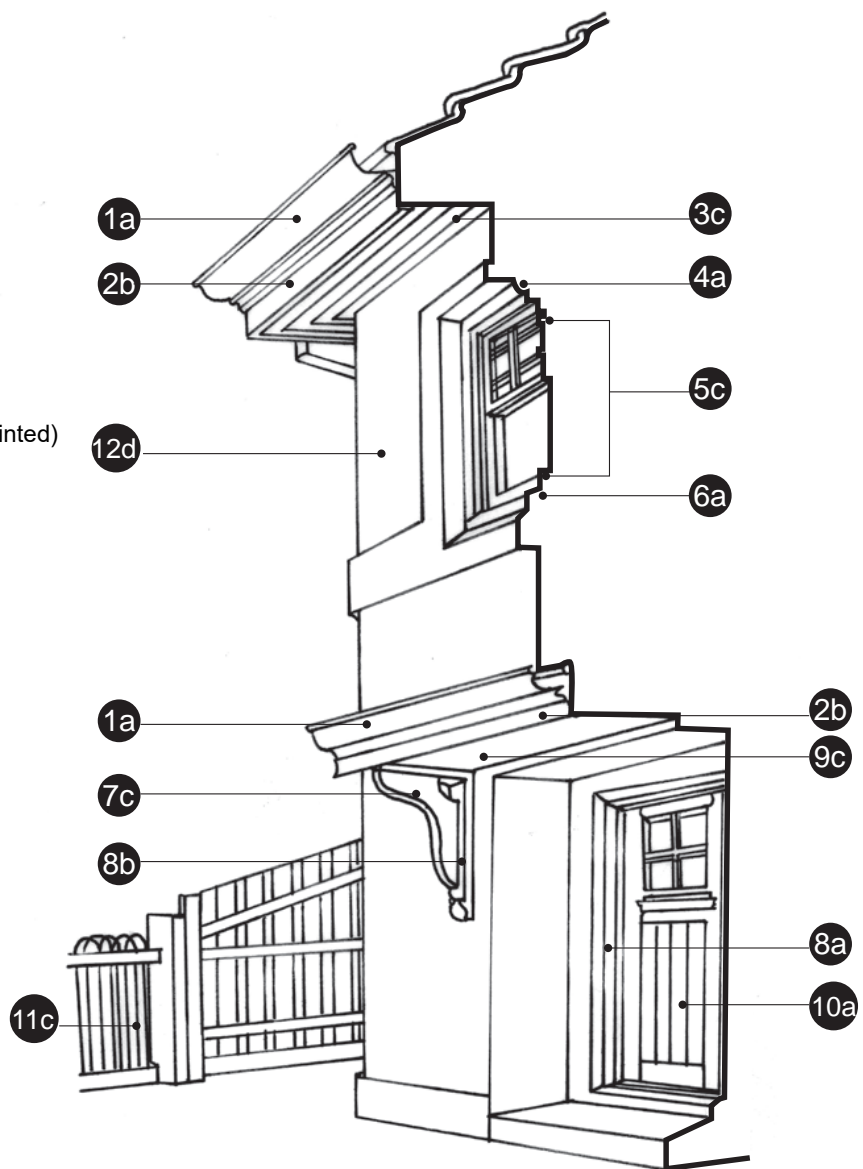
Figure 4. Facade articulations
